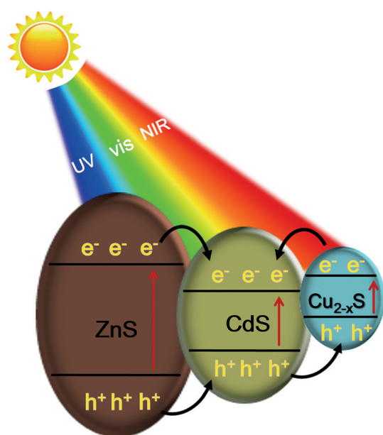
Scheme 1. Energy band alignment and the flow of photogenerated carriers in the ZnS–CdS– \text{Cu}_{2-x}\text{S} nanosystem. The ZnS–CdS– \text{Cu}_{2-x}\text{S} ternary hybrid material effectively absorbs UV, visible, and NIR light. The photogenerated electrons flow to the conduction band of CdS in this hybrid system while the hole carriers mostly accumulate at the valence band of \text{Cu}_{2-x}\text{S} .
